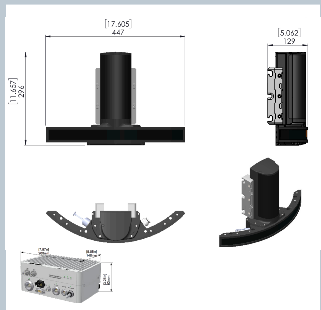
Sonar incl bracket (bracket shown in grey)
